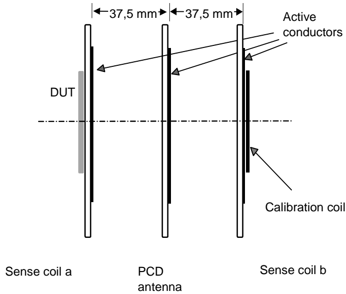
Figure 3 — Test PCD assembly
