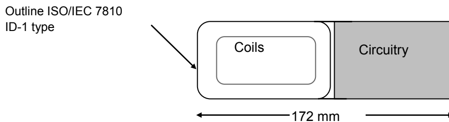
Figure 4 — Reference PICC dimensions
