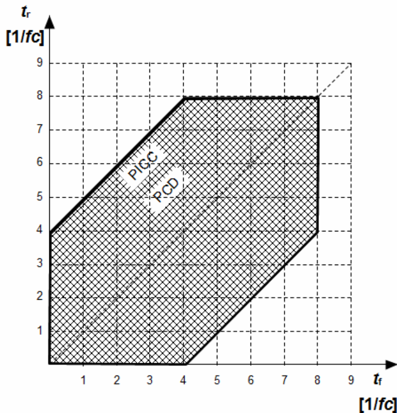
Figure 17 — Type B modulation waveform timing parameters for a bit rate of fc/16
