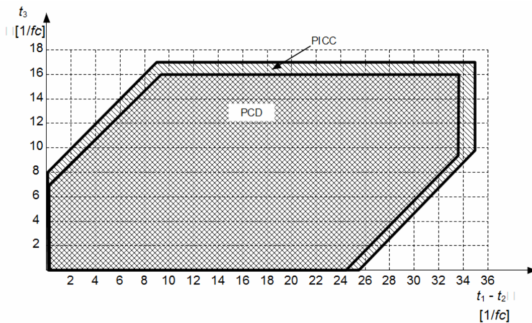
Figure 4 — Type A modulation waveform timing parameters for a bit rate of fc/128
