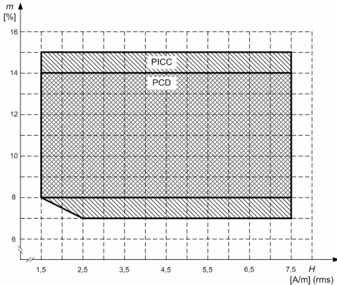
Figure 13 — Type B modulation index m for bit rates of fc/128 , fc/64 , fc/32 and fc/16
