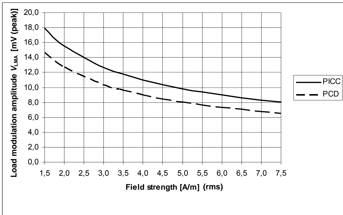
Figure 11 — Load modulation amplitude
