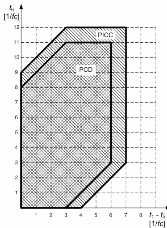
Figure 7 — Type A modulation waveform timing parameters for a bit rate of fc/64
