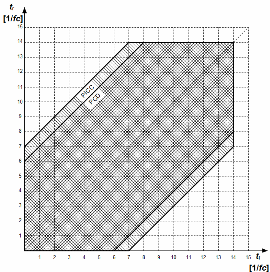
Figure 15 — Type B modulation waveform timing parameters for a bit rate of fc/64
