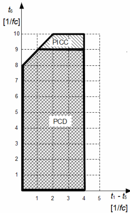
Figure 8 — Type A modulation waveform timing parameters for a bit rate of fc/32
