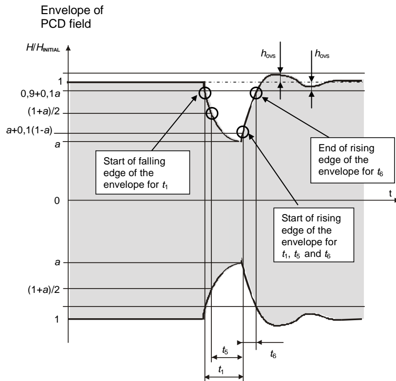
Figure 6 — PauseA for bit rates of fc/64 , fc/32 and fc/16
