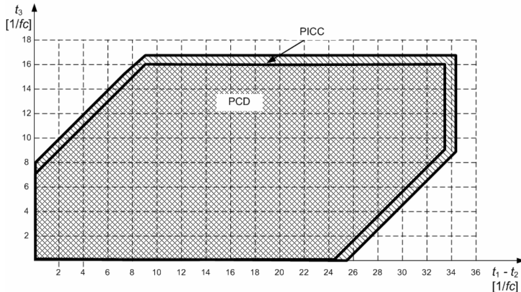
Figure 4 — Type A modulation waveform timing parameters for bit rate of fc/128
