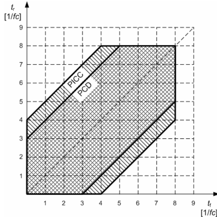
Figure 17 — Type B modulation waveform timing parameters for a bit rate of fc/16
