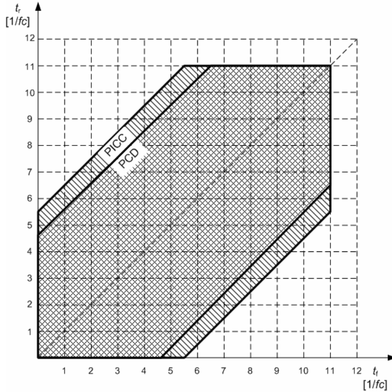
Figure 16 — Type B modulation waveform timing parameters for a bit rate of fc/32
